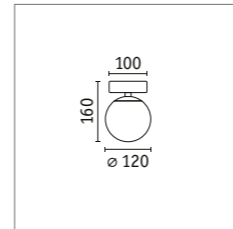
Gove Wall and ceiling luminaire IP44 71064 □ p. 50
