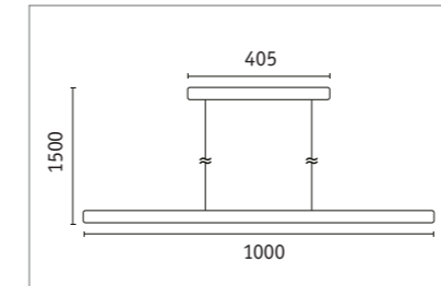
Lento Ceiling luminaire 79693 □ p. 55
