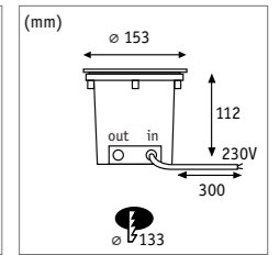
Durea 140 Recessed luminaire IP67 94654 □ p. 56
