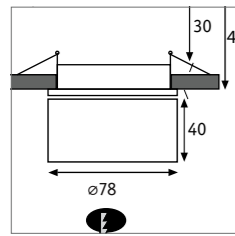
Spircle Recessed luminaire 93374 □ p. 54
