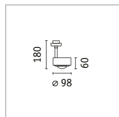
Aldan URail spot 95519 □ p. 53
