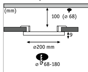
Veluna VariFit Edge Recessed panel luminaire IP44 79957 □ p. 50
