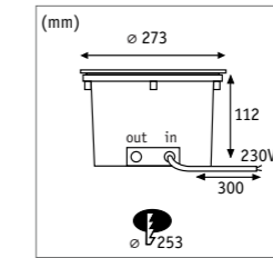
Durea 260 Recessed luminaire IP67 94656 □ p. 56
