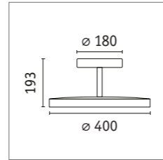
Hildor Ceiling luminaire 96781 □ p. 54
