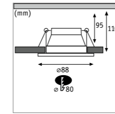
Cole Recessed luminaire 93397 □ p. 54
