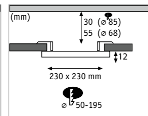
Areo VariFit Recessed panel luminaire 79967 □ p. 54
