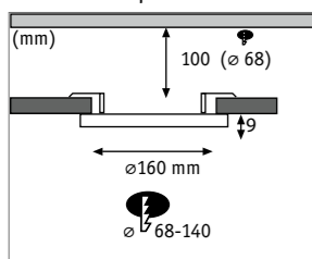
Veluna VariFit Edge Recessed panel luminaire IP44 79956 □ p. 50
