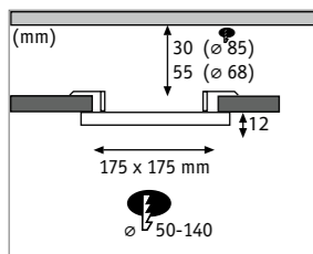
Areo VariFit Recessed panel luminaire 79966 □ p. 54
