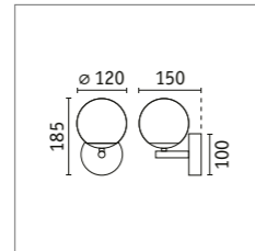
Gove Wall luminaire IP44 71067 □ p. 50
