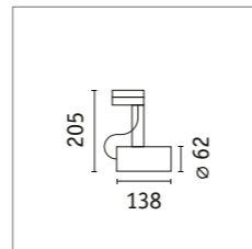
Apol ProRail3 spot 95410 □ p. 51
