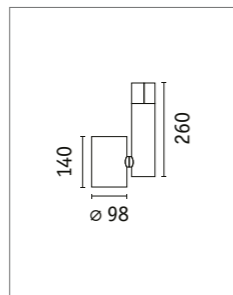
Zeuz URail Spot 95537 □ p. 52
