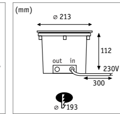
Durea 200 Recessed luminaire IP67 94655 □ p. 56
