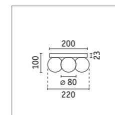
Gove Wall and ceiling luminaire IP44 71069 □ p. 51
