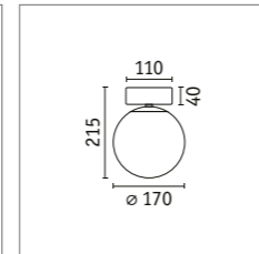
Gove Wall and ceiling luminaire IP44 71065 □ p. 50
